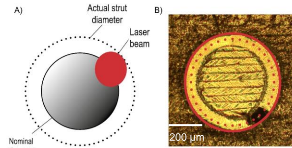
Fig 5. a) Nominal and actual diameter representative illustration (contribution of the laser beam to final strut diameter). b) The measurement procedure (dashed line is laser beam path, continuous line is measured path).
