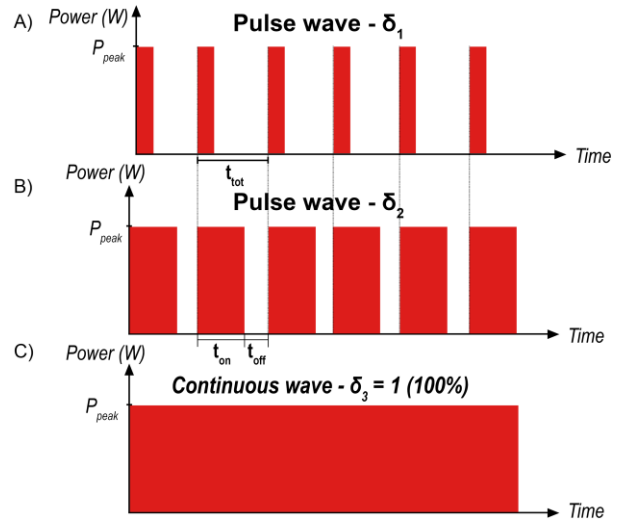
Fig 1. Theoretical temporal pulse shapes: Perfect temporal profiles. a) PW-low duty cycle with total pulse time ( t_{tot} ). b) PW-high duty cycle with laser-on ( t_{on} ) and laser-off ( t_{off} ) times. c) CW- with \delta = 100\% .
