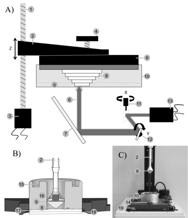
Figure 1: Schematic principle of the used stereolithography configuration A) original machine setup Nobel 1.0; B) CAD data modified chamber and modified building platform; C) photograph of the modified setup at Nobel 1.0 including a sample (8) [9]
