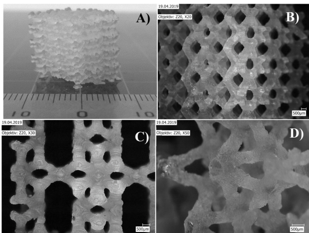
Figure 4: Representation of the filigree structure of the scaffold, A) overview, B) diagonal view, C) detail with continuous channels, D) filigree structure of a strut
