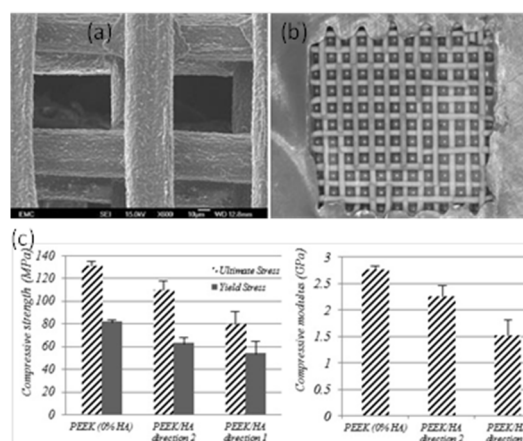
Figure 3 (a) 3D printed HA scaffolds with filament as fine as 50 μm, (b) produced bioactive PEEK/HA composite, and (c) the results of compression test on the PEEK/HA samples (c)
