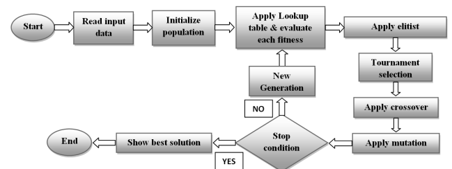
Figure 1. The genetic code to obtain the optimal parameters.
