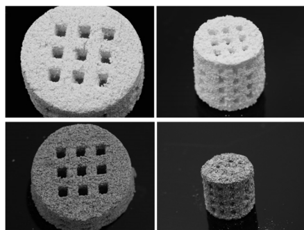
Figure 1: Interconnected porous scaffolds of BaTiO 3 -composite (50:50) after 3D printing (top) and sintering (bottom.)
