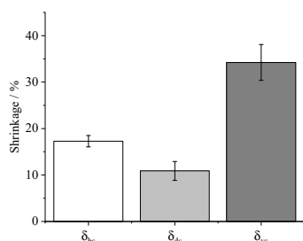
Figure 2: Influence of the sintering in terms of linear shrinkage in different directions and in volume.
